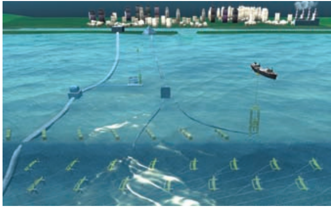
A rendering of an aerial view showing ocean energy technology installed offshore Florida to provide electricity, hydrogen, and cold water cooling generated from the Gulf Stream and ocean thermal energy. Florida Atlantic University - Center for Ocean Energy Technology
